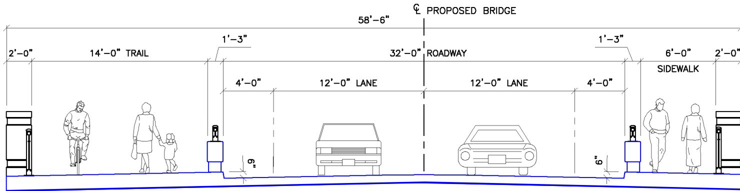
Revised Bridge Cross Section 2 Lane Bridge with Sidewalk (east side) and Path (west side)
